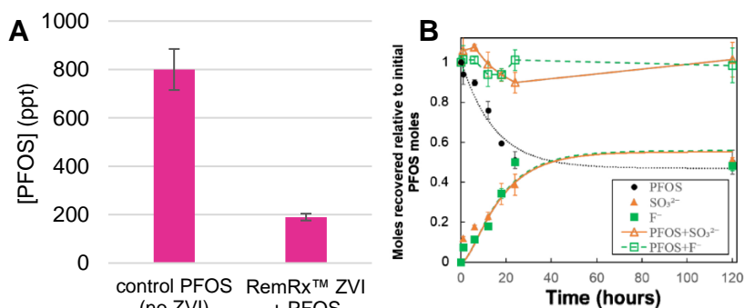
FIGURE 4. (A) PFOS removal by RemRx™ ZVI compared to a control after 24 hours at 50 °C. (B) PFOS mass balance in a reaction containing NiFe nanoparticles on activated carbon at 60 °C. The sum of relative moles of sulfite and fluoride with residual PFOS achieves near mass balance (reproduced from ref. 10).
