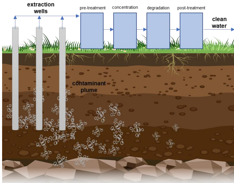
FIGURE 2. A representative PFAS treatment train. PFAS is extracted from groundwater and passed through subsequent treatment stages, including pre-treatment (e.g. adjustment of hydrological conditions), concentration through selective sorption agents, degradation, and post-treatment to prepare the effluent for discharge.
